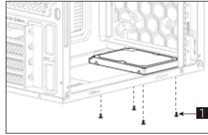
(5c) Install 2.5" SSD x1
