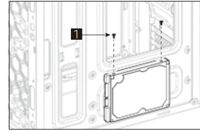
(5d) Install 2.5" SSD x1
